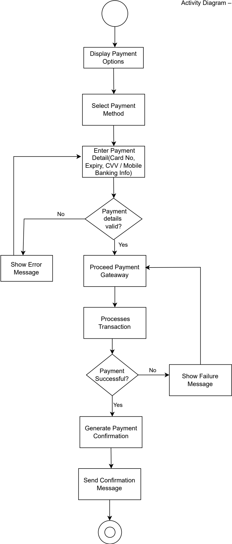
Activity Diagram – Payment Process
